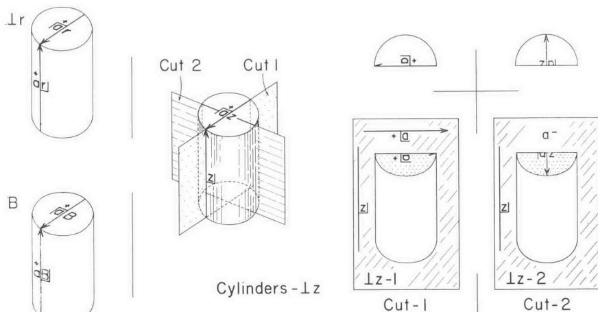
Fig. 5. Conventions for marking the orientation of crystals and thin sections. Marks on cylinders 1r and B are shown on the left. On the right are the two types of thin section cut from a 1z cylinder and the stages in the preparation and marking of the thin section: top, half of the cylinder ground away; bottom, the half-cylinder mounted on marked slide ready for grinding and finishing.
